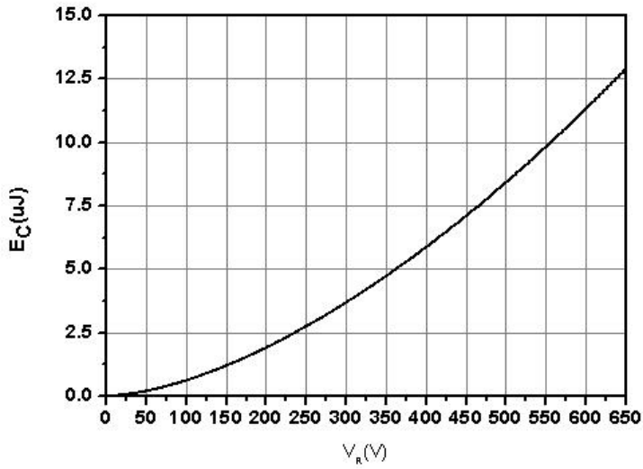
Fig.5-Capacitance Stored Energy
