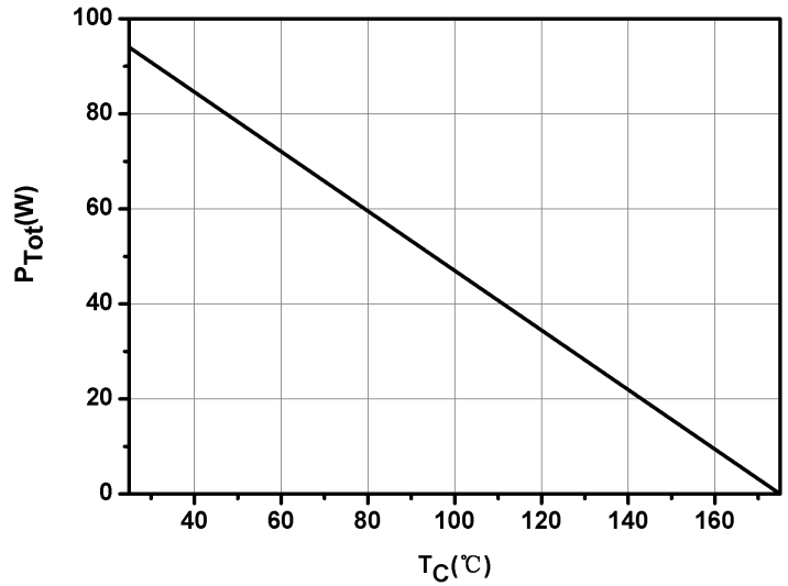
Fig.6-Power Derating
